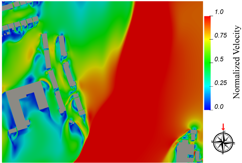
Figure 7.2: Ground Floor Level - Flow Velocity Results at Z=1.5m above the ground - Wind Direction: 0°
