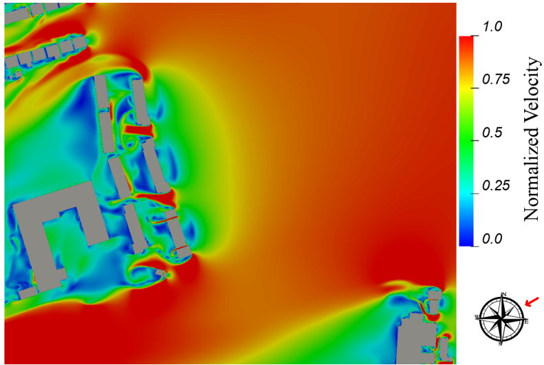
Figure 7.4: Ground Floor Level - Flow Velocity Results at Z=1.5m above the ground - Wind Direction: 60°
