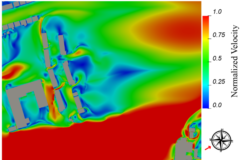
Figure 7.10: Ground Floor Level - Flow Velocity Results at Z=1.5m above the ground - Wind Direction: 240°
