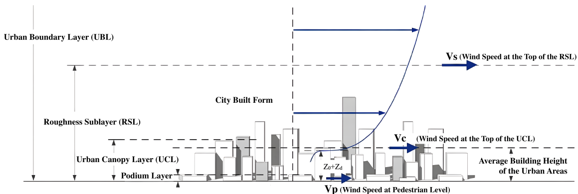
Figure 2.4: Wind Velocity Profile
