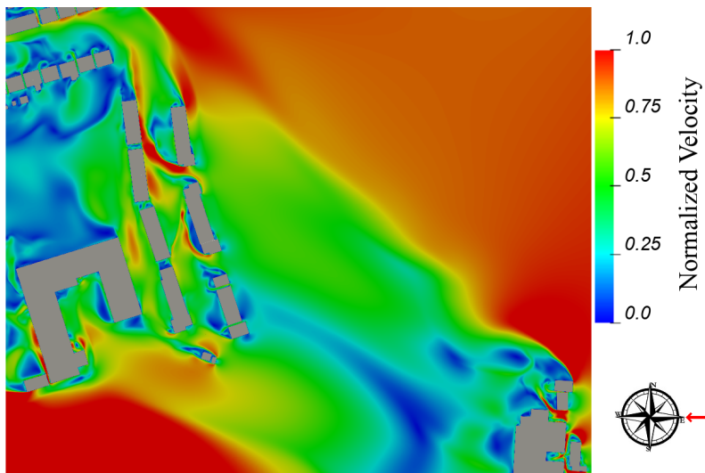
Figure 7.5: Ground Floor Level - Flow Velocity Results at Z=1.5m above the ground - Wind Direction: 90°
