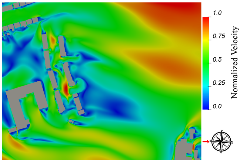
Figure 7.11: Ground Floor Level - Flow Velocity Results at Z=1.5m above the ground - Wind Direction: 270°
