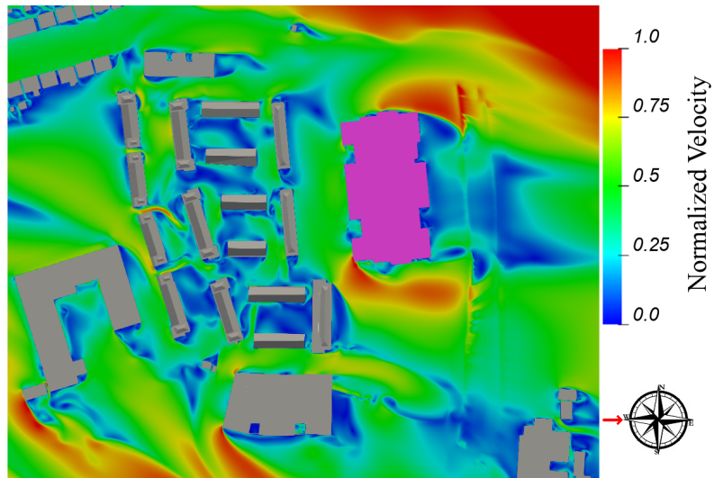
Figure 8.11: Ground Floor Level - Flow Velocity Results at Z=1.5m above the ground - Wind Direction: 270°
