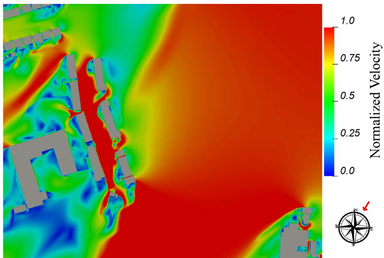
Figure 7.3: Ground Floor Level - Flow Velocity Results at Z=1.5m above the ground - Wind Direction: 30°
