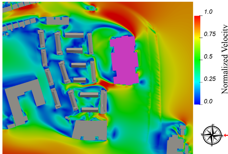
Figure 8.5: Ground Floor Level - Flow Velocity Results at Z=1.5m above the ground - Wind Direction: 90°
