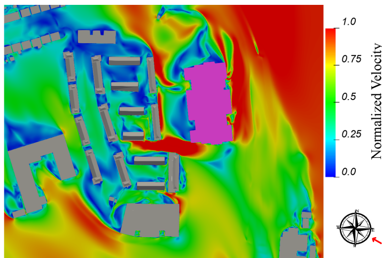
Figure 8.6: Ground Floor Level - Flow Velocity Results at Z=1.5m above the ground - Wind Direction: 120°
