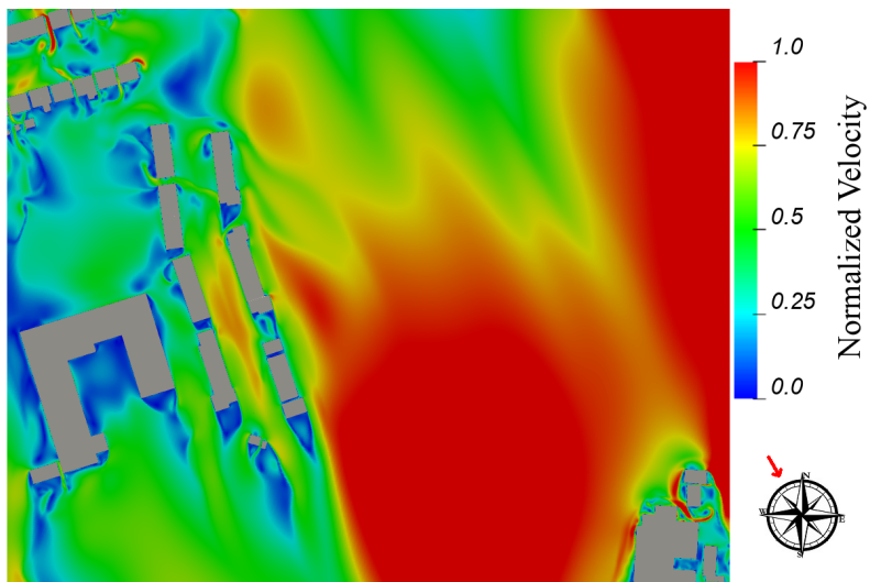
Figure 7.13: Ground Floor Level - Flow Velocity Results at Z=1.5m above the ground - Wind Direction: 330°
