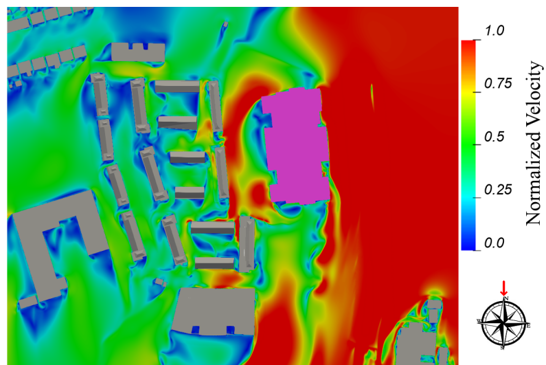
Figure 8.2: Ground Floor Level - Flow Velocity Results at Z=1.5m above the ground - Wind Direction: 0°
