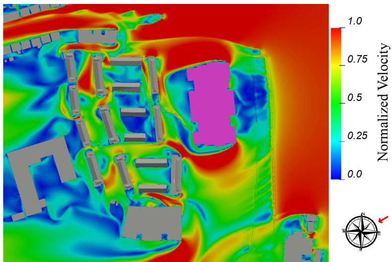
Figure 8.4: Ground Floor Level - Flow Velocity Results at Z=1.5m above the ground - Wind Direction: 60°
