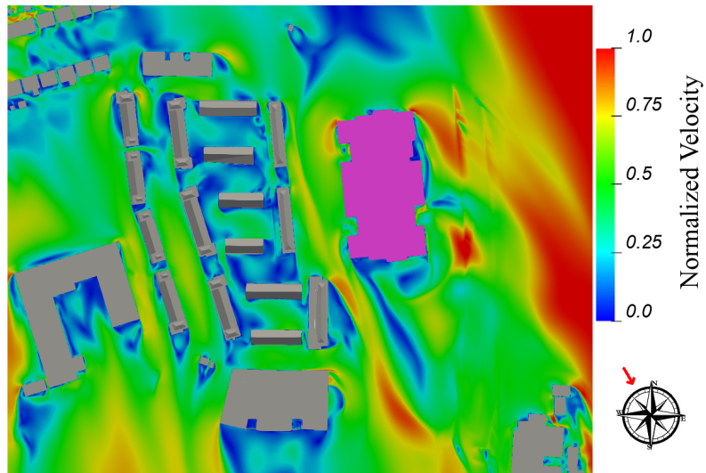
Figure 8.13: Ground Floor Level - Flow Velocity Results at Z=1.5m above the ground - Wind Direction: 330°
