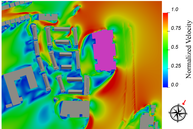
Figure 8.3: Ground Floor Level - Flow Velocity Results at Z=1.5m above the ground - Wind Direction: 30°
