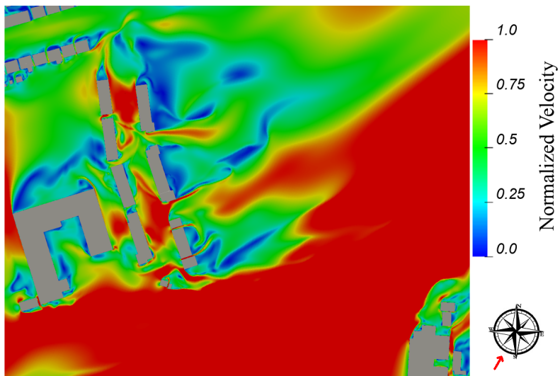
Figure 7.9: Ground Floor Level - Flow Velocity Results at Z=1.5m above the ground - Wind Direction: 210°
