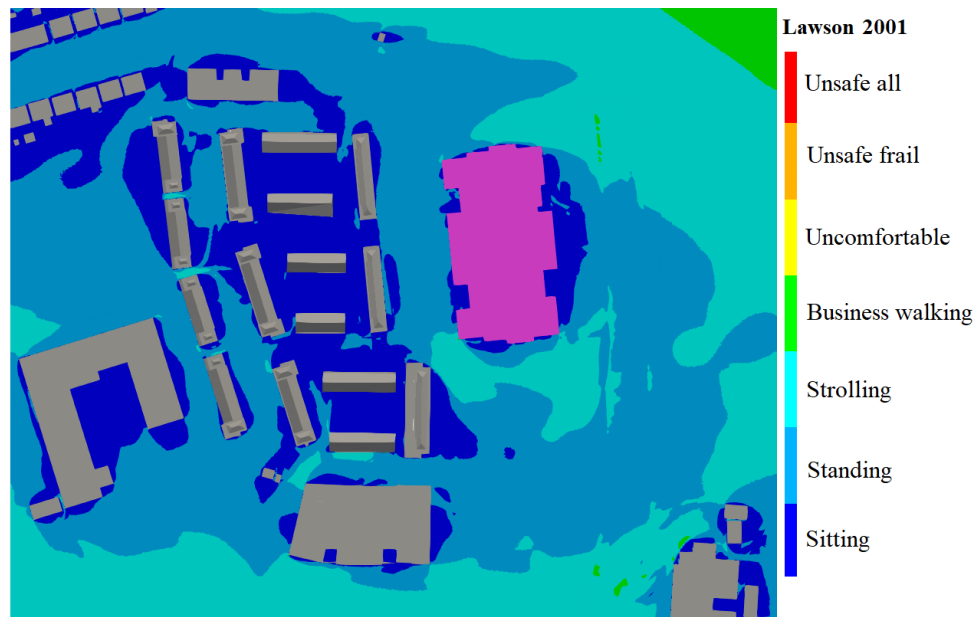
Figure 8.14: Ground Floor - Lawson Discomfort Map - Top View
