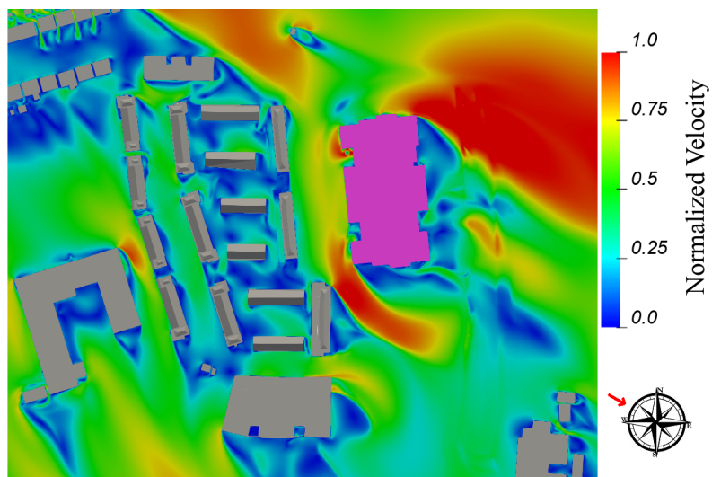
Figure 8.12: Ground Floor Level - Flow Velocity Results at Z=1.5m above the ground - Wind Direction: 300°
