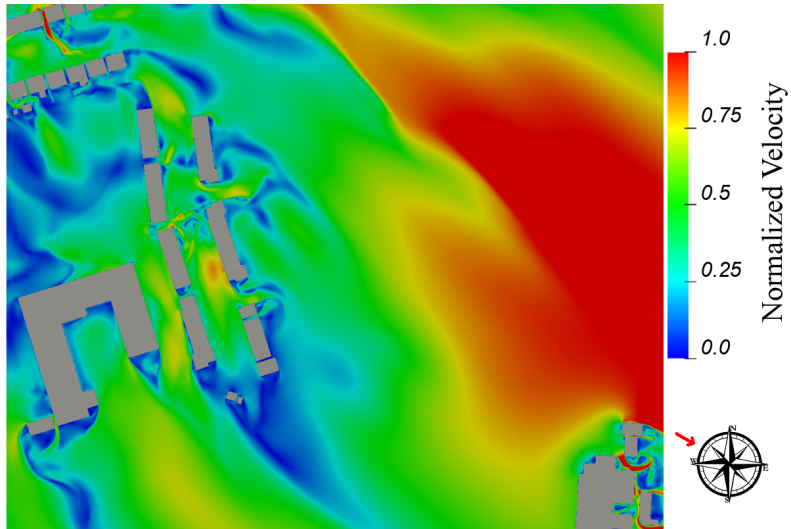
Figure 7.12: Ground Floor Level - Flow Velocity Results at Z=1.5m above the ground - Wind Direction: 300°
