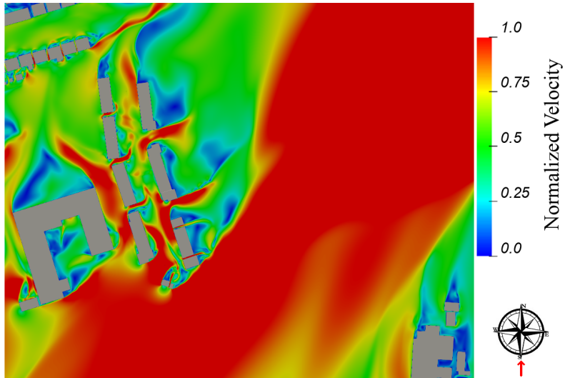
Figure 7.8: Ground Floor Level - Flow Velocity Results at Z=1.5m above the ground - Wind Direction: 180°
