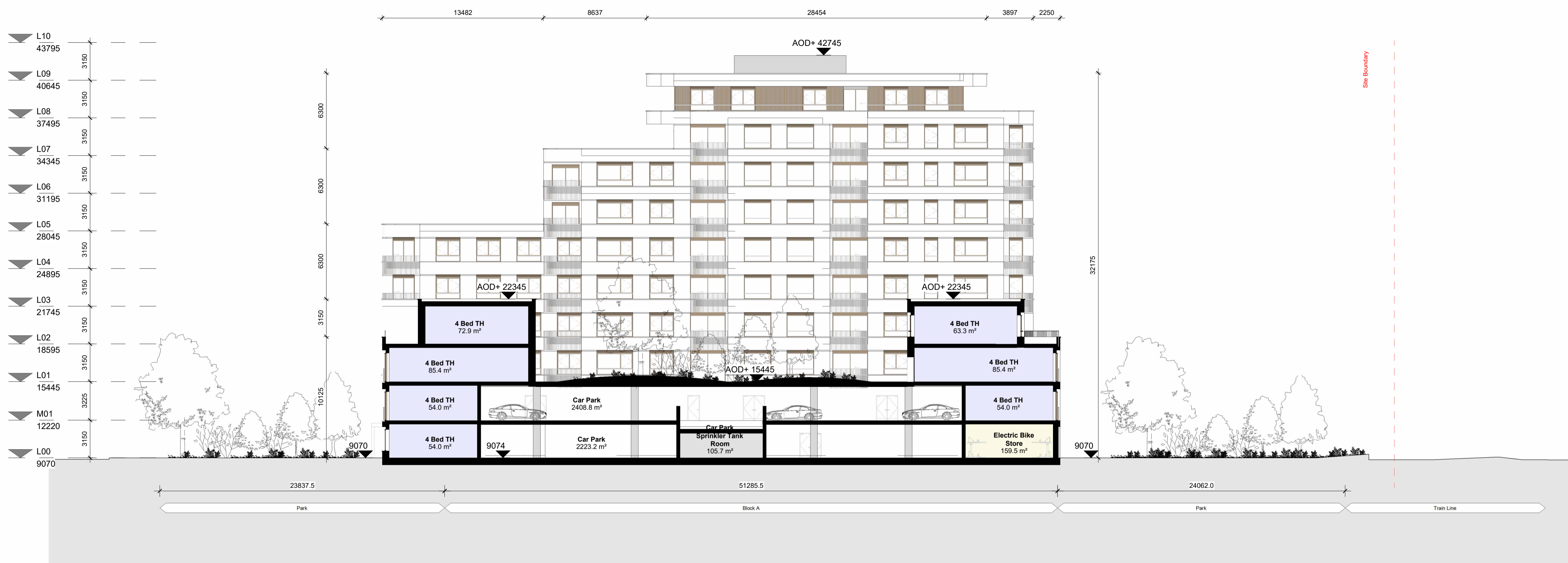
Block A Section CC 1 : 200
