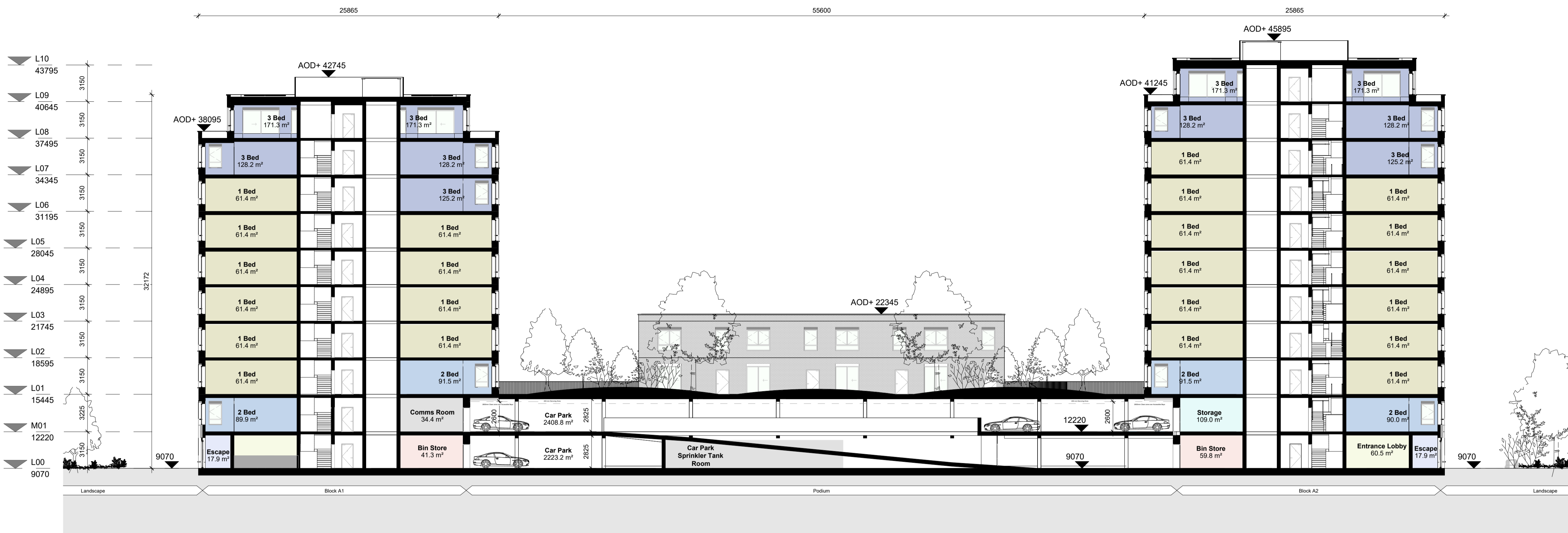
Block A Section AA 1: 200
