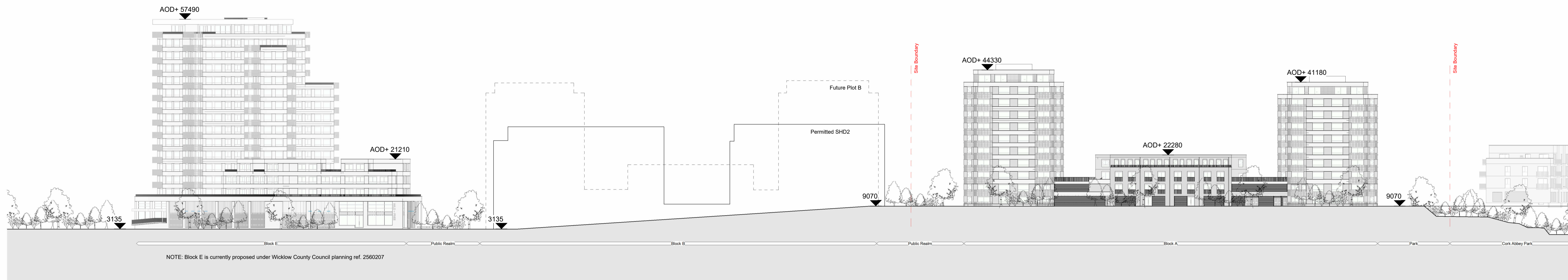
Site Elevations 01 1:500
